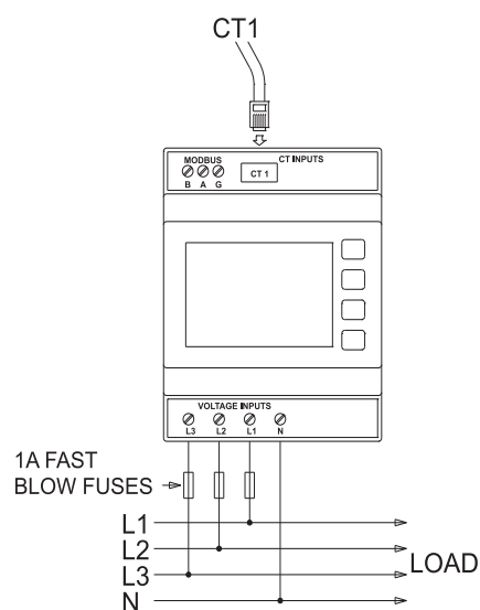
3 phase, 4-wire
