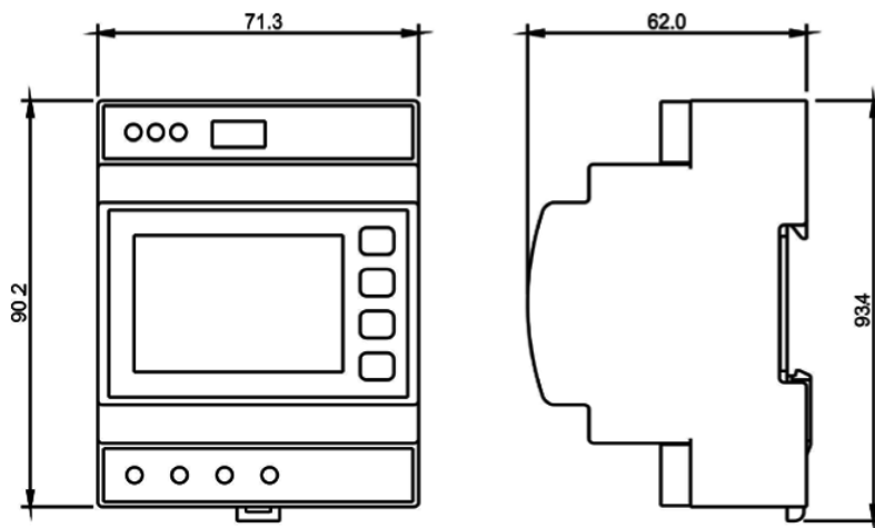
Single-phase, 2-wire
