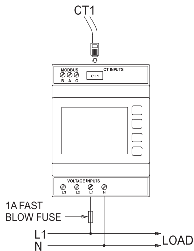
Single-phase, 2-wire
